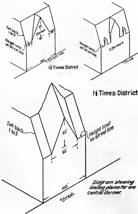
FIG. 1 NEW YORK CITY ZONE LAW DIAGRAMS
